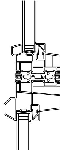
Horizontal Standard Mull to Double Hung
