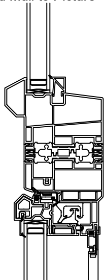
Horizontal Windowwall Mull
