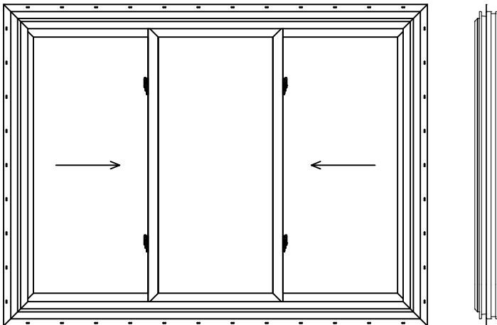
Basic Frame - 3 Lite End Vent Unit -(Equal Lite 1/3-1/3-1/3) (XOX)
