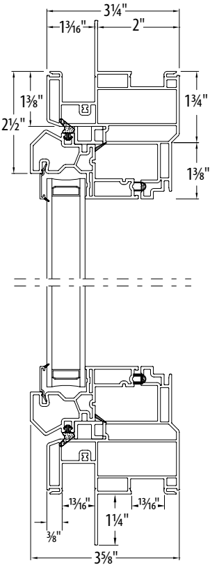
Casement Picture (Fixed) Cross-Sectional Head and Sill Detail
