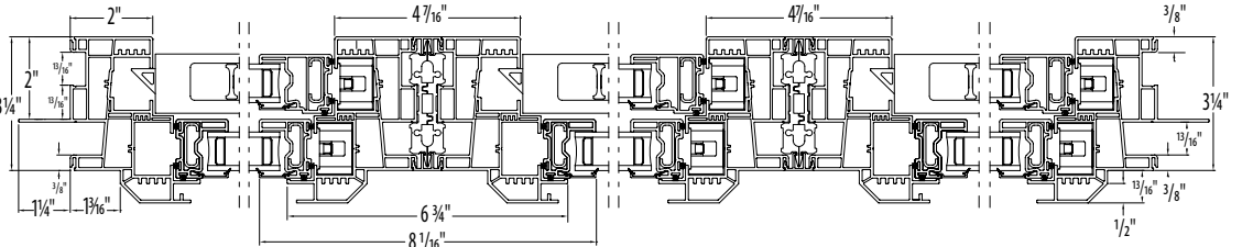
Triple Double-Hung 3U1R3C ® Horizontal Detail
