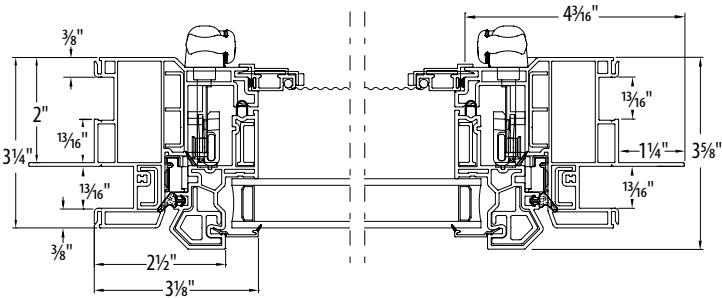
Awning Cross-Sectional Jamb Detail
