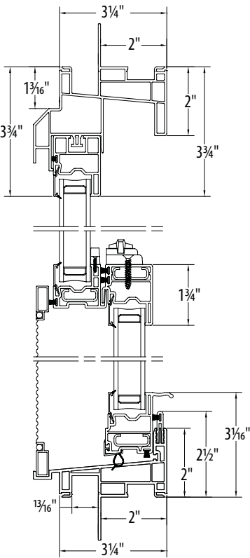
Single-Hung Vertical Detail
