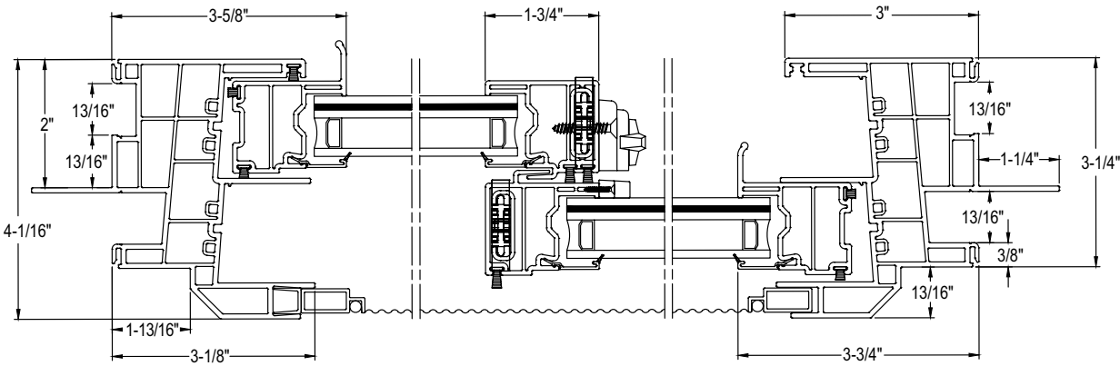
2-Lite Slider Horizontal Detail
