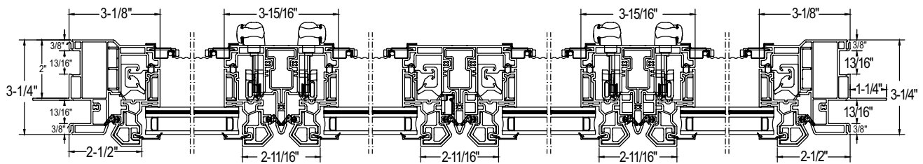
Casement/Picture/Casement Horizontal Detail
