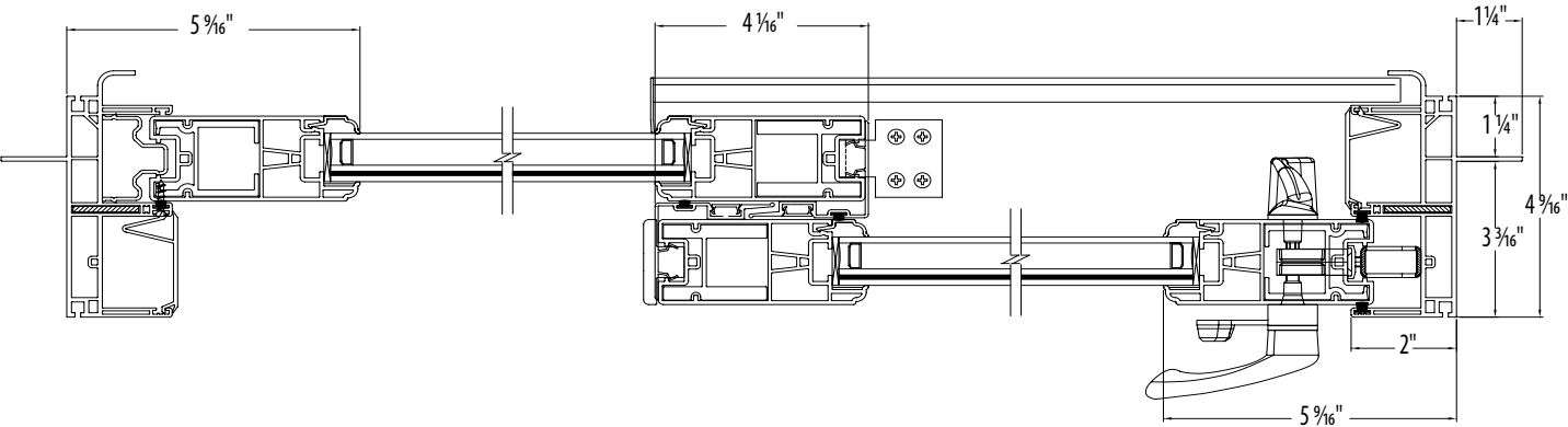
Patio Door Cross-Sectional Jamb Detail
