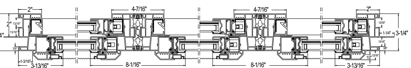
Triple Double-Hung 3U1R3C ® Horizontal Detail
