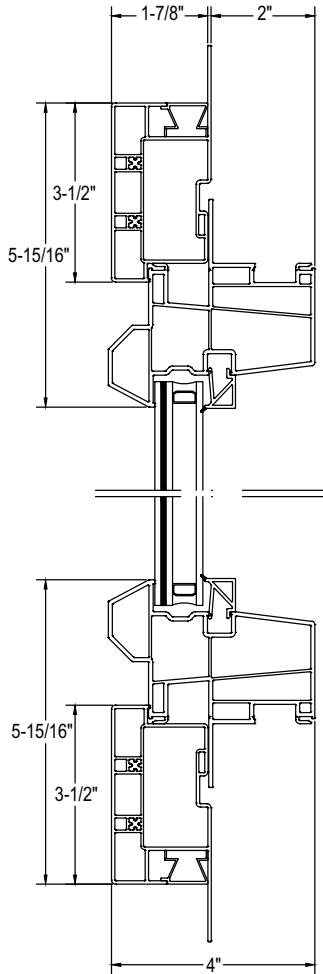
3.5" Flat Casing w/o Pocket Filler Horizontal Detail
