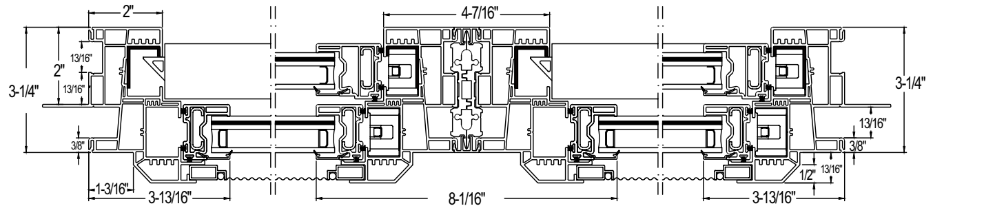
Triple Double-Hung 3U1R3C ® Horizontal Detail
