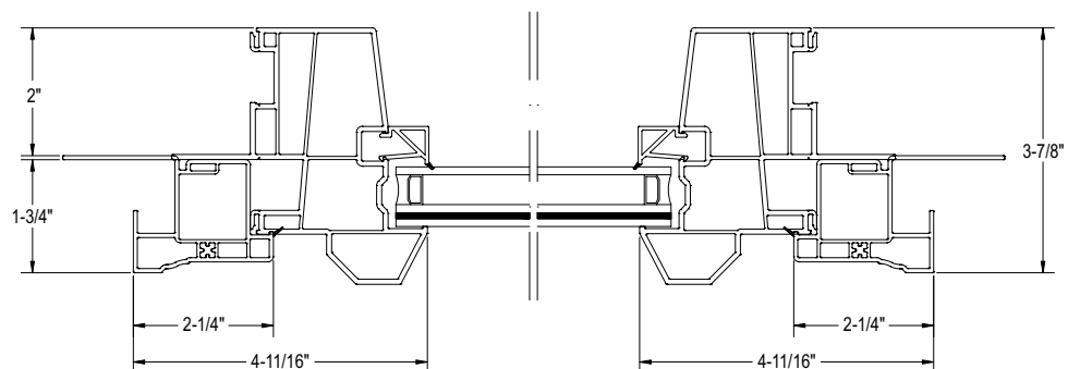
Brick Mold Casing w/o Pocket Filler Horizontal Detail
