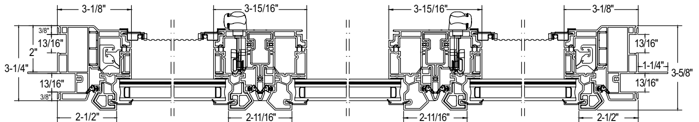
Casement/Picture/Casement Horizontal Detail
