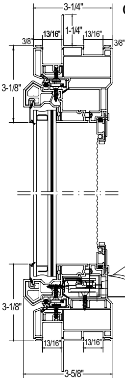
Casement Cross-Sectional Head & Sill Detail
