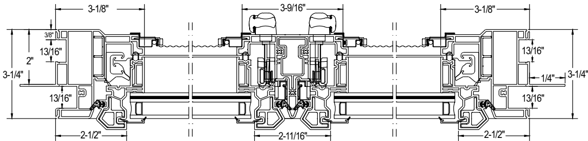
Twin Casement Cross-Sectional Jamb Detail with Integral Mullion
