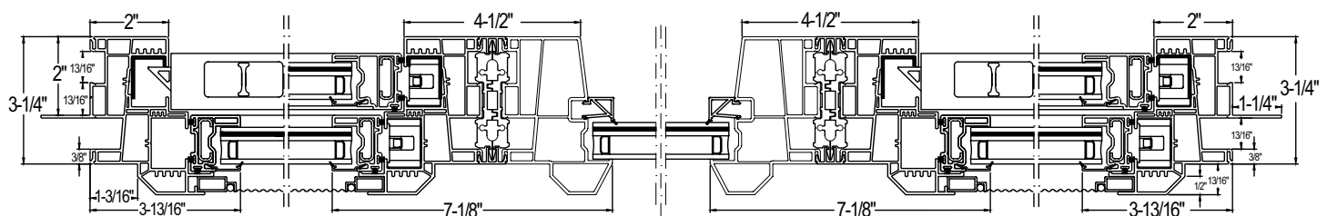
Double-Hung/ Picture/Double-Hung 3U1R3C® Horizontal Detail
