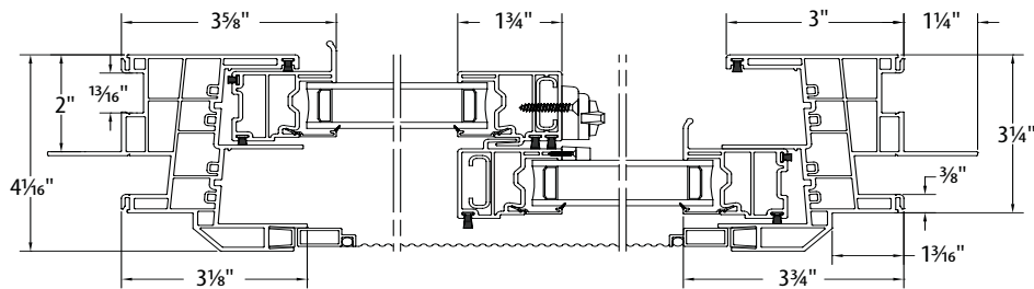
2-Lite Slider Horizontal Detail
