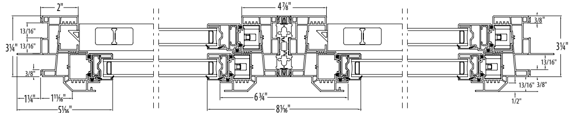
Twin Double-Hung 2U1R2C ® Horizontal Detail
