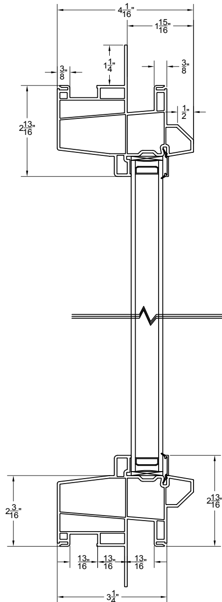
Picture & Transom Vertical Detail
