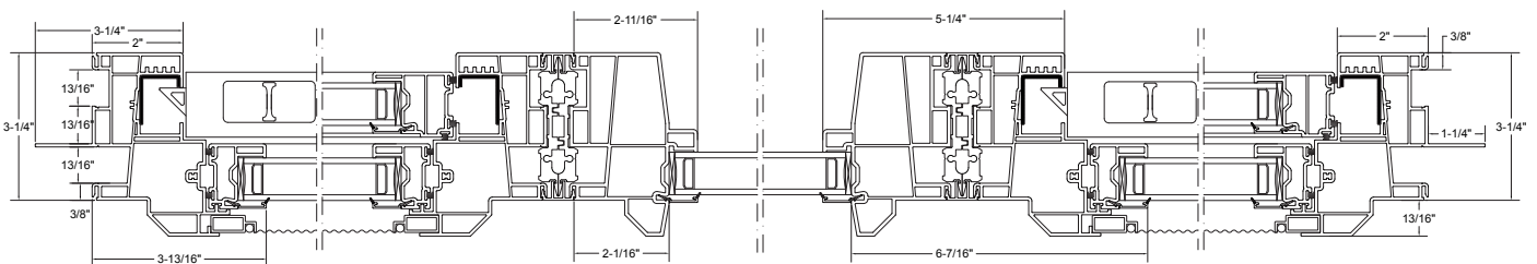
Single-Hung/Picture/Single-Hung 3U1R3C ® Horizontal Detail
