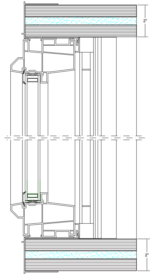
10° Bow Window Vertical Detail
