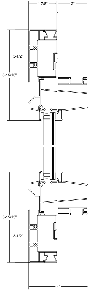
3.5" Flat Casing Picture Frame w/ Pocket Filler Vertical Detail
