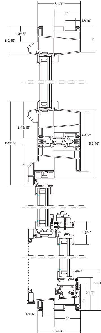
Single-Hung with Transom 2U2R1C ® Vertical Detail
