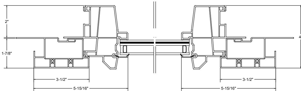
3.5" Flat Casing w/o Pocket Filler Horizontal Detail
