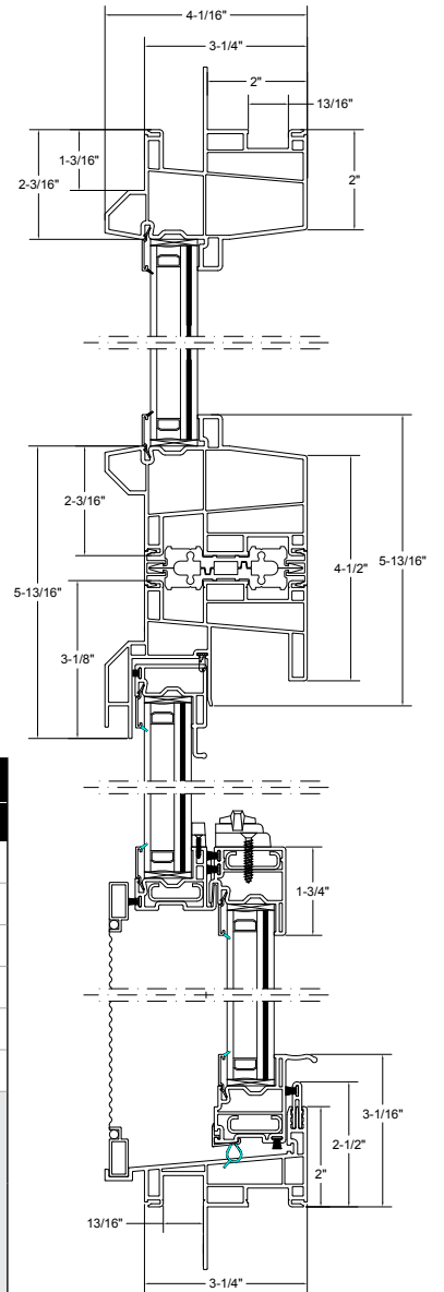
Double-Hung with Transom 2U2R1C ® Vertical Detail
