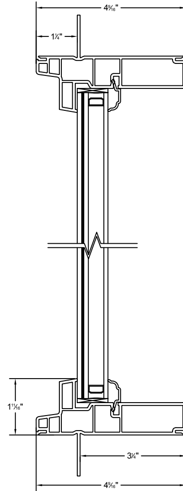
Sidelites and Transoms Vertical Detail
