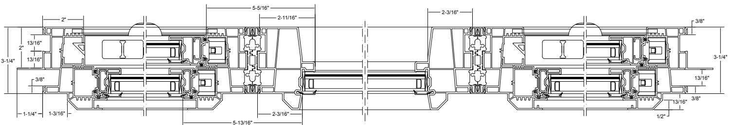
Double-Hung/ Picture/Double-Hung 3U1R3C ® Horizontal Detail
